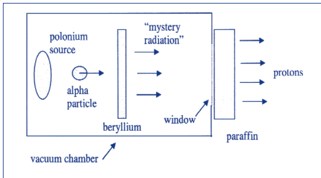
Figure 1 The “beryllium radiation” experiment of Becker, Bothe, the Joliot-Curies and Chadwick.
