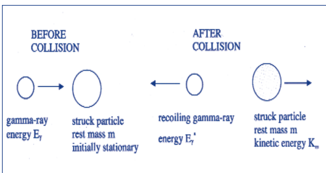
Figure 2 A gamma-ray strikes a stationary massive particle, setting it in motion. The gamma-ray is assumed to recoil backwards.
